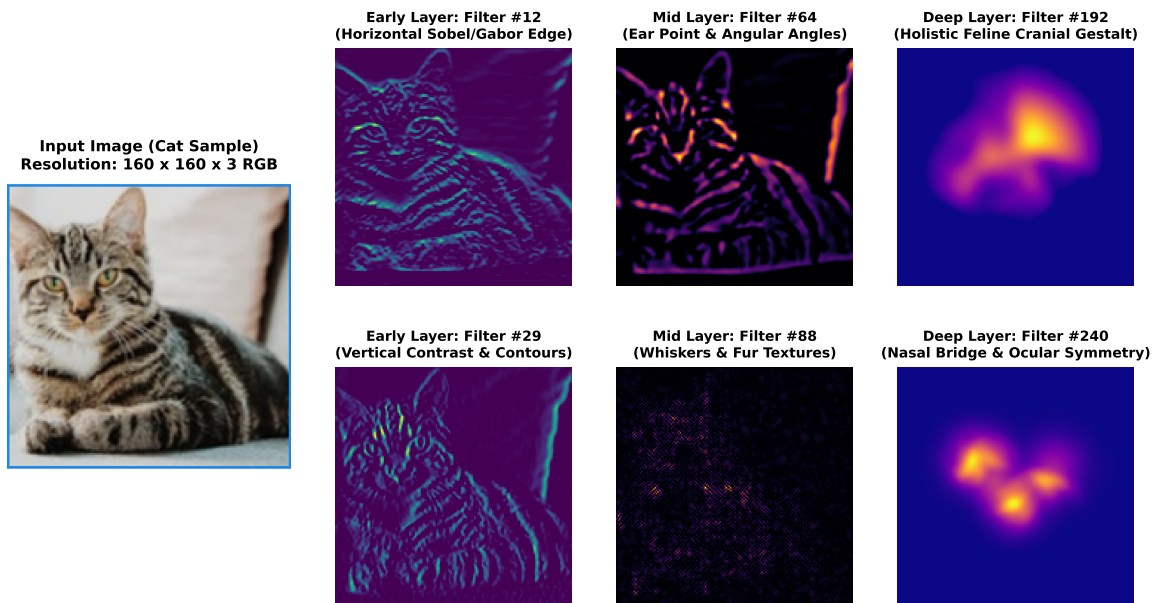
Model-derived MobileNetV2 activations.
